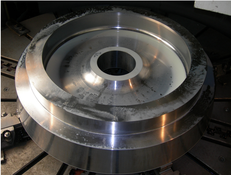
Turbocharger Disk for gas turbine Ø 1400 mm.
