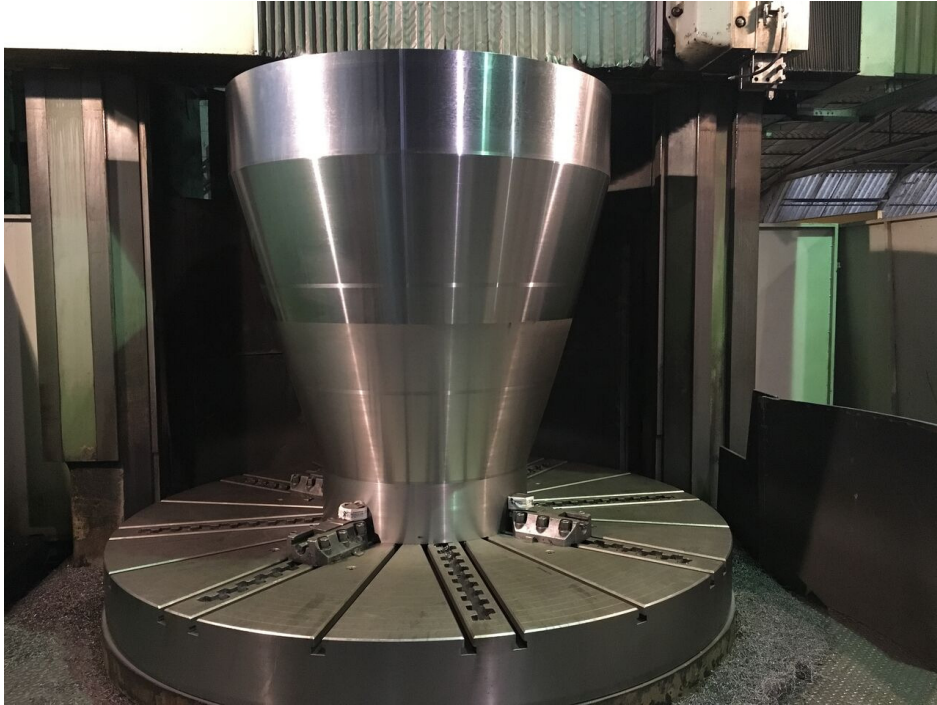
Fuselage Mold
