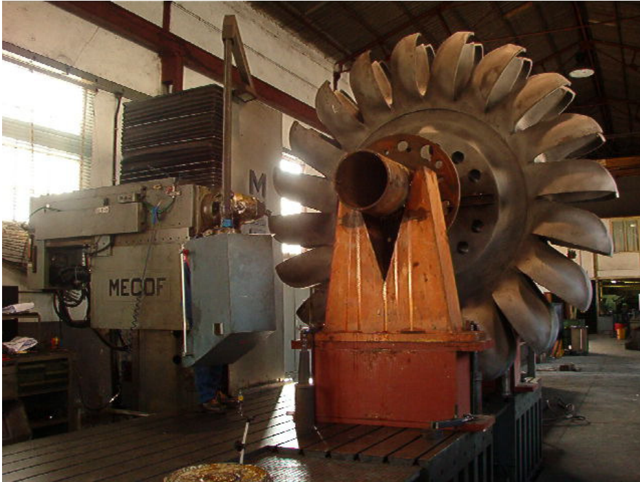
Pelton Turbine
